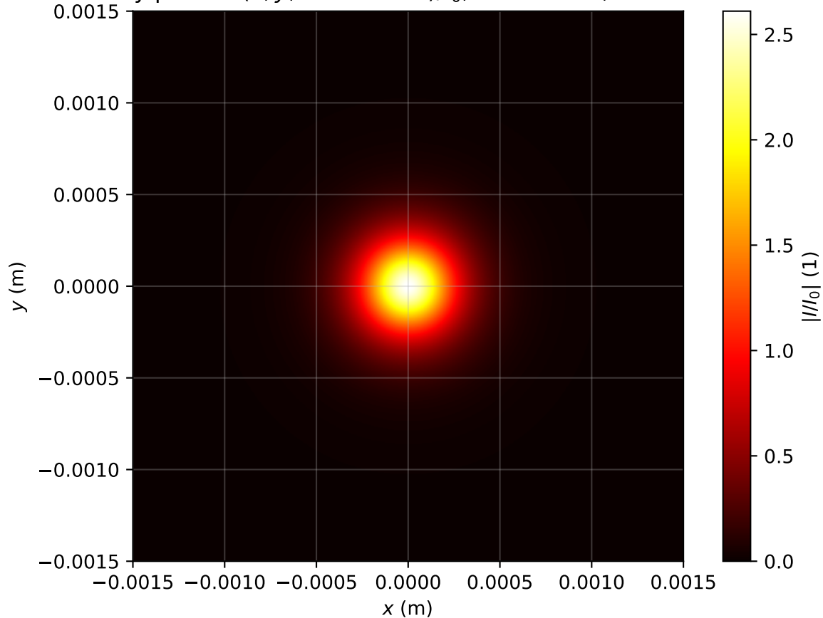
Intensity profile I(x, y, z = 2.946m)/I_0 , Pin=1.0Pcr, artificial time
